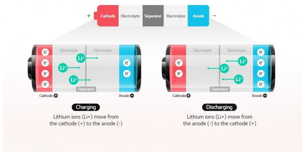
Figure 10- Lithium- Ion Battery Cross Section
